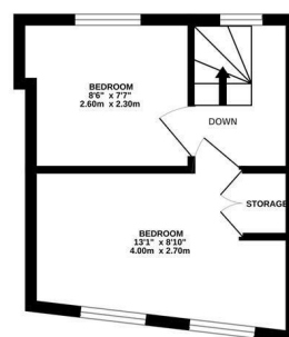
1ST FLOOR 200 sq.ft. (18.6 sq.m.) approx.
